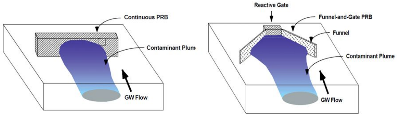
Permeable Reactive Barrier (PRB) technology for remediating contaminated ground water (EPA, 1998)
